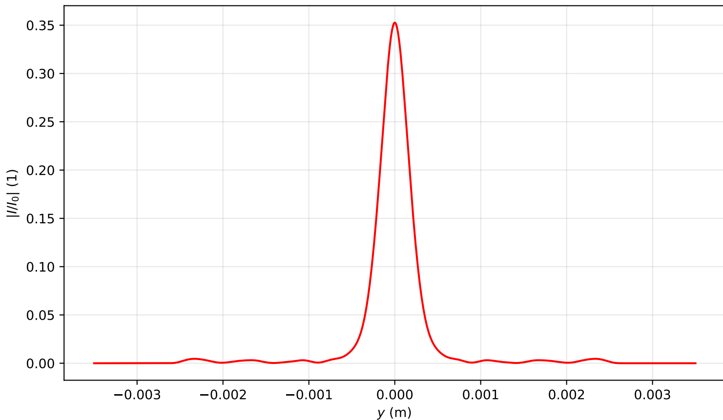
Intensity profile I(x=0, y, z=3.662)/I_0 , P_{in}=7.0P_{cr} , artificial time
